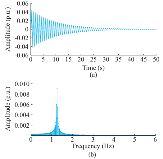
Fig. 3. \Delta P_e(t) and its Fourier transform. (a) \Delta P_e(t) in time domain. (b) Amplitude-frequency characteristic of \Delta P_e(t) in frequency domain.
