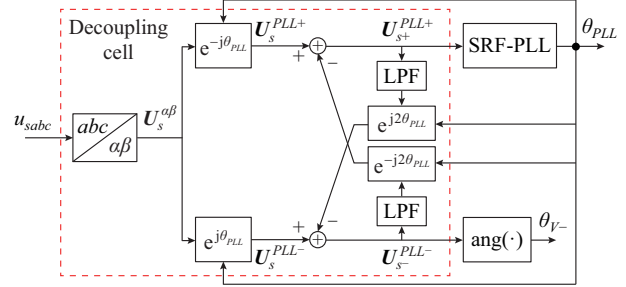
Fig. 6. Basic block diagram of DDSRF-PLL.
